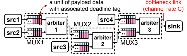
Figure 3: A three-node queueing network with perfect priority queues with infinite capacity. Dotted rectangles are a network component called “MUX”, which merges two incoming flows into a single outgoing one. Each packet carries an associated deadline and the priority queue can dequeue the packet having the earliest deadline. The arbiter and the priority queue are assumed to have zero-cycle delay, which implies a packet just generated at any source can be immediately forwarded to the sink at channel rate C through the combinational path if the packet wins all arbitrations on the path.
